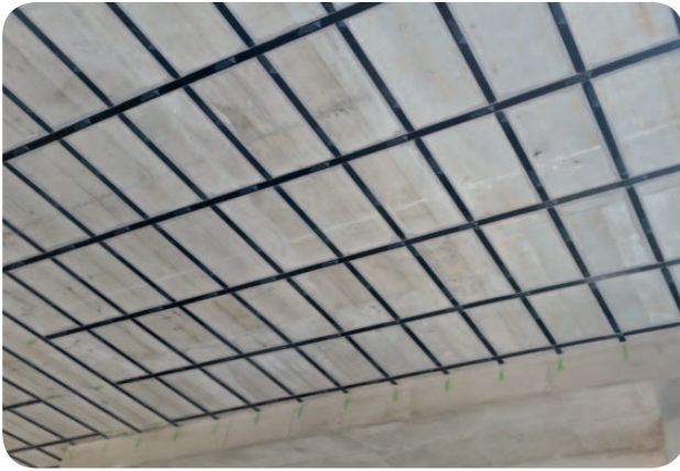
Fig. 17 Carbon fiber reinforced lamellas before fire protection
